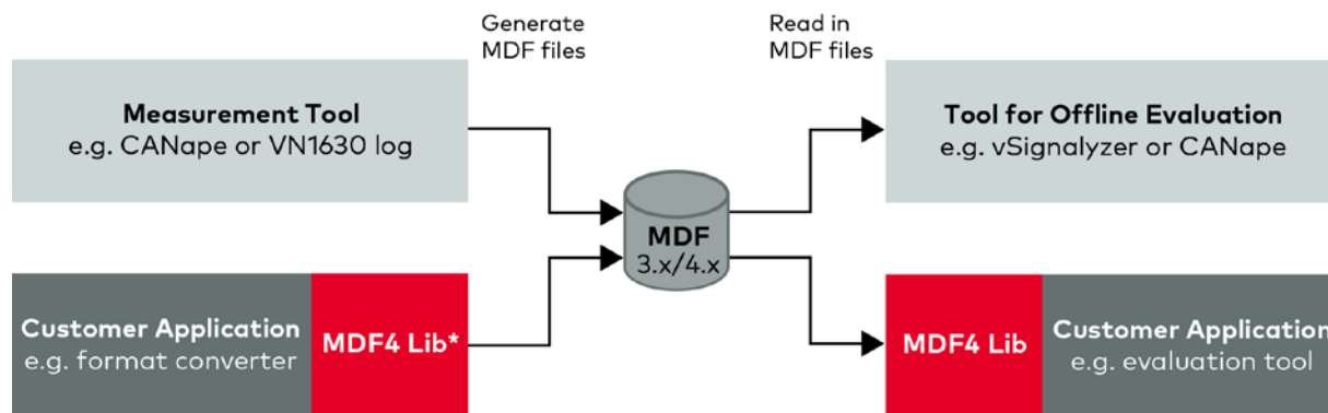
Figure 1: Function library MDF4 Lib integrates measurement data formats like MDF3 and MDF4 easily and quickly in your applications.
